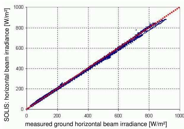
Fig. 8. Horizontal direct-beam irradiance evaluated by SOLIS versus the correspondent ground measurements.
