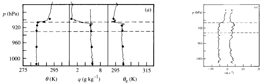
Well-mixed Sc layer
