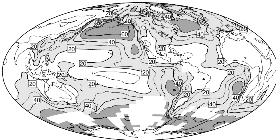
Klein and Hartmann (1993), from surface observations
