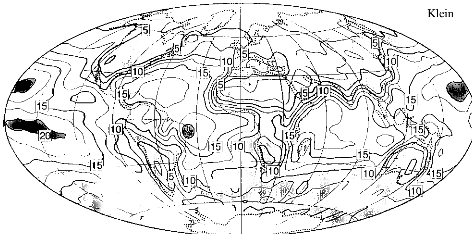
Cumulus Cloud Amount
