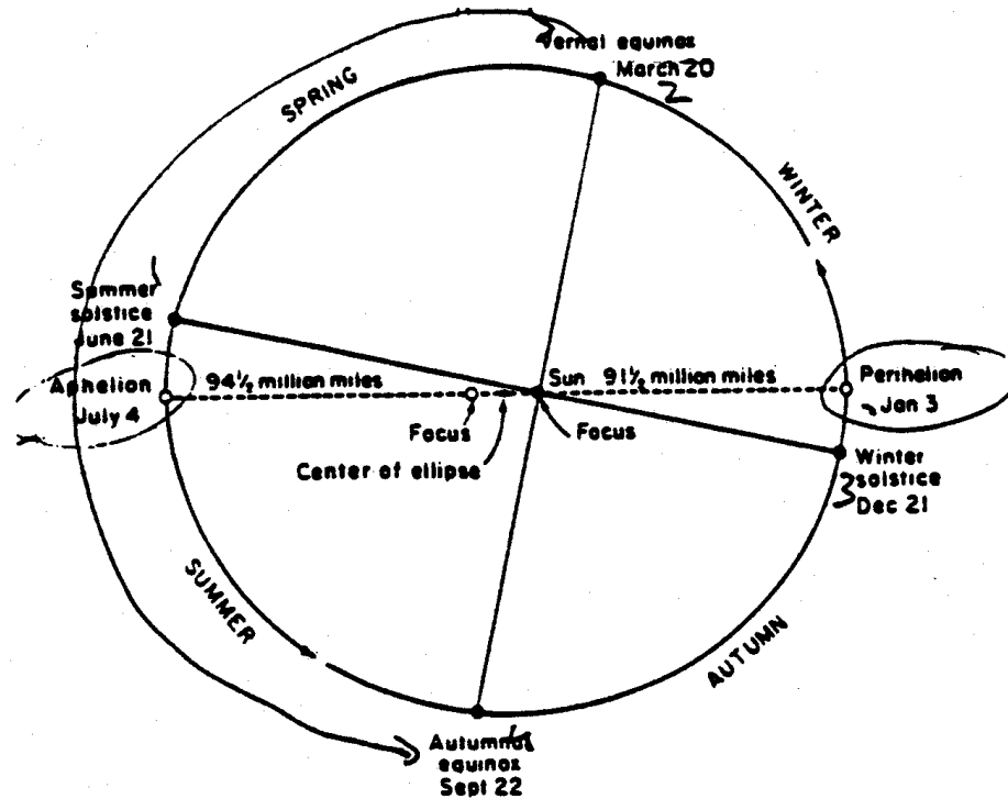
Fig. 5.4 Dates of equinox and solstice. At the equinoxes, the Earth's axis is pointed at right angles to the sun, and the day and night are of equal length all over the globe. At the summer solstice, the North Pole is tipped in the direction of the sun and the northern hemisphere has the longest day of the year. At the winter solstice, the North Pole is tipped away from the sun, and the northern hemisphere has the shortest day of the year.
